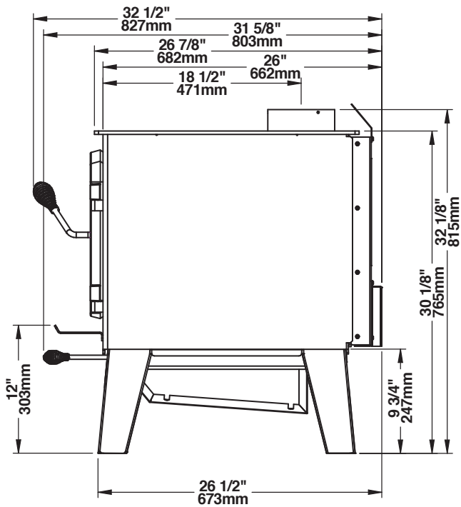
Figure 3: Side View
