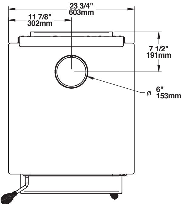
Figure 1: Top View
