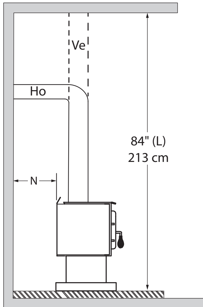
Figure 18: Clearances - Side
