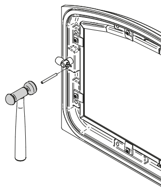
Figure 25: Installing the split pin
