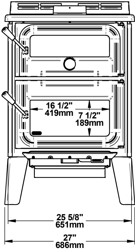
Figure 2: Front view
