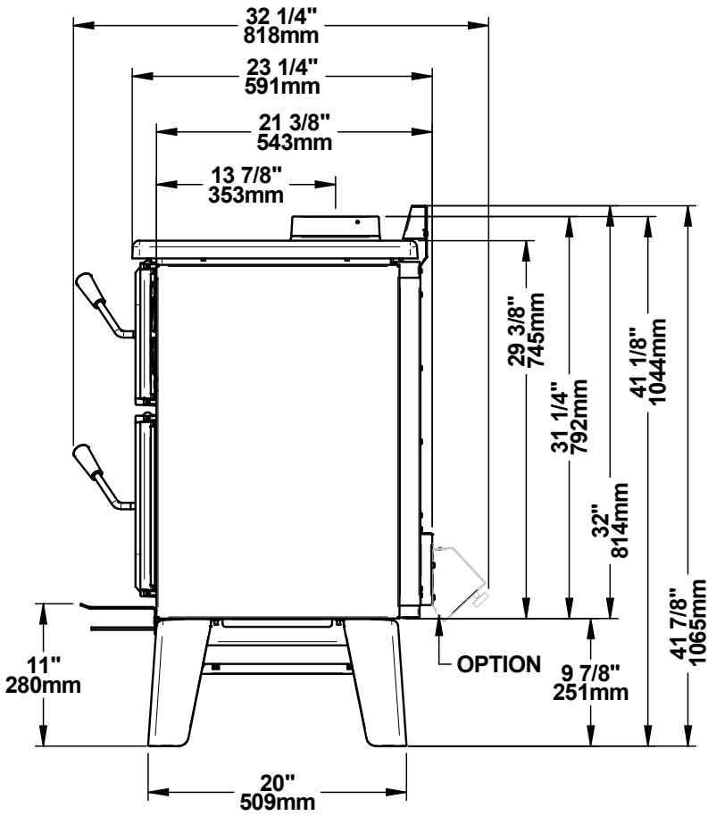
Figure 3: Side view
