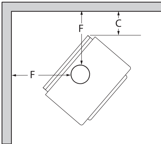
Figure 37: Clearances - Corner
