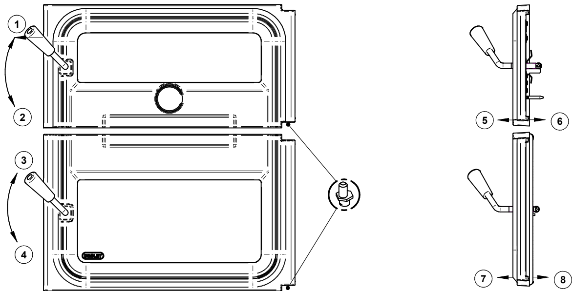
Figure 31: Eccentric hinges depth adjustment
