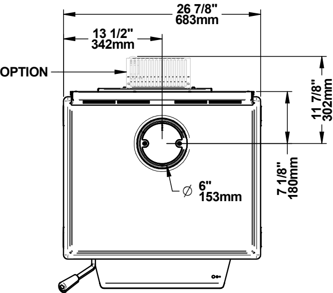
Figure 1: Top view
