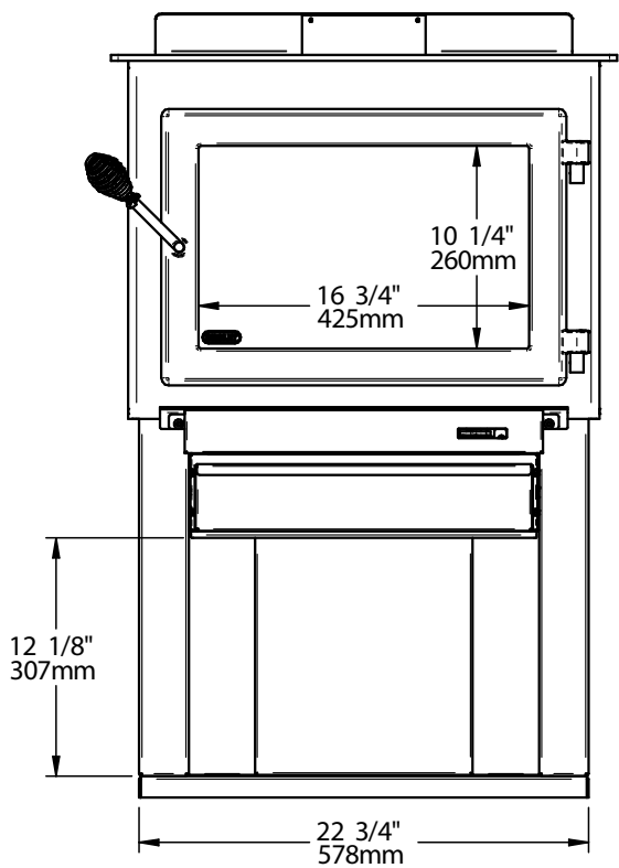
Figure 2: Front View
