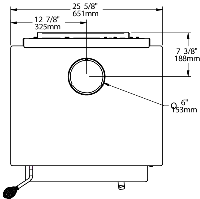
Figure 1: Top View
