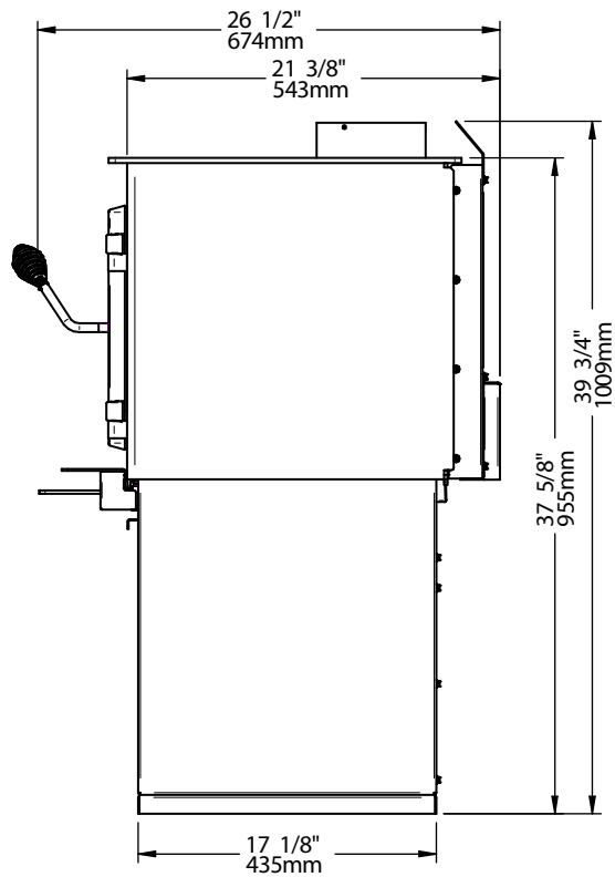
Figure 3: Side View
