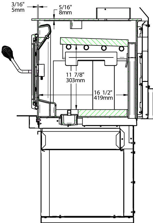
Figure 6: Side View - Combustion Chamber
