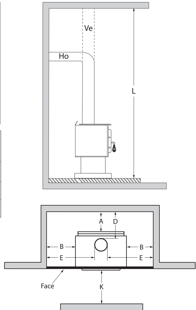
Figure 13: Clearances -Alcove
