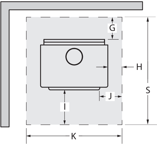
Figure 16: Floor Protection
