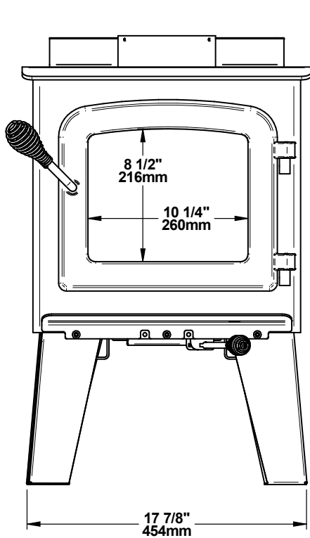
Figure 2: Front View
