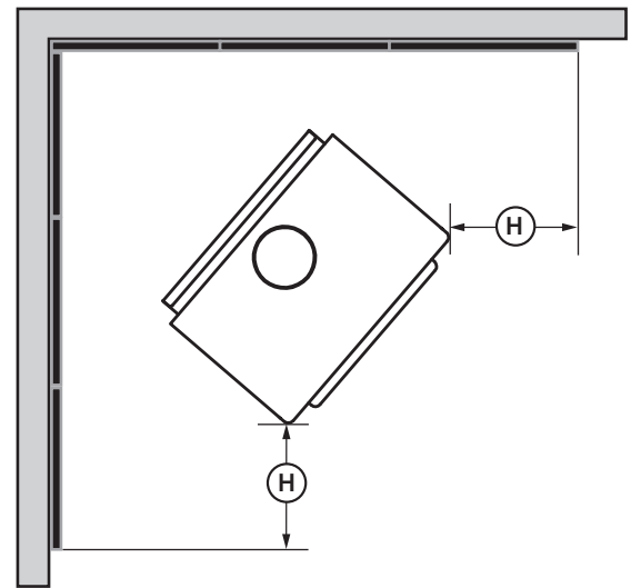
Figure 20: Heat shield clearances
