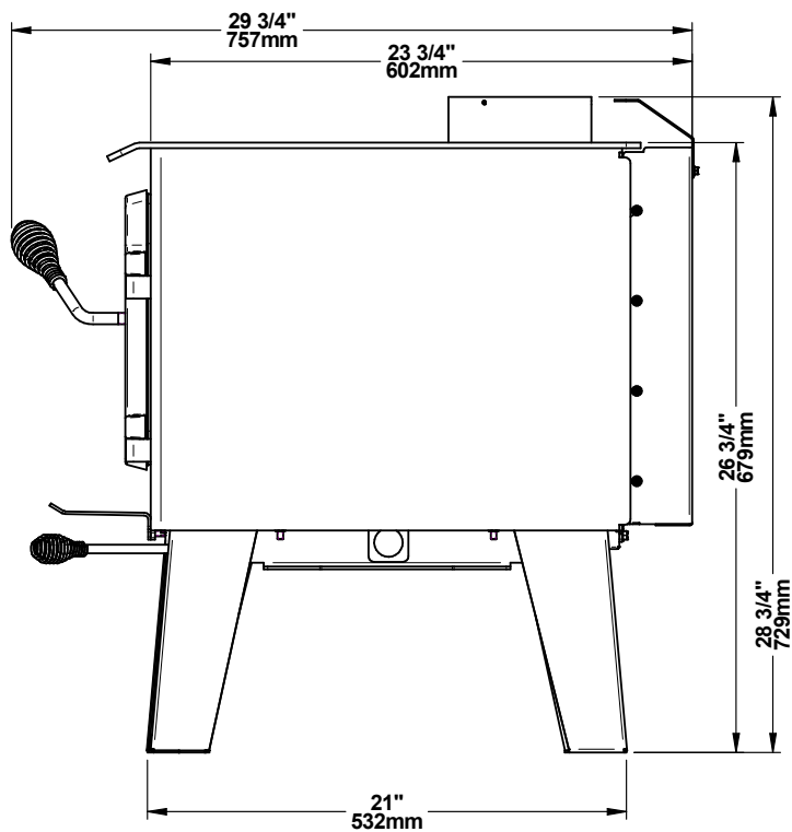
Figure 3: Side View
