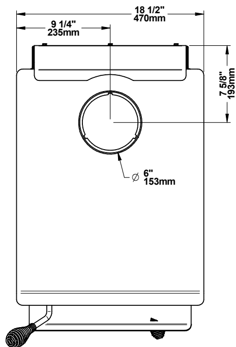
Figure 1: Top View
