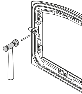
Figure 22: Installing the split pin
