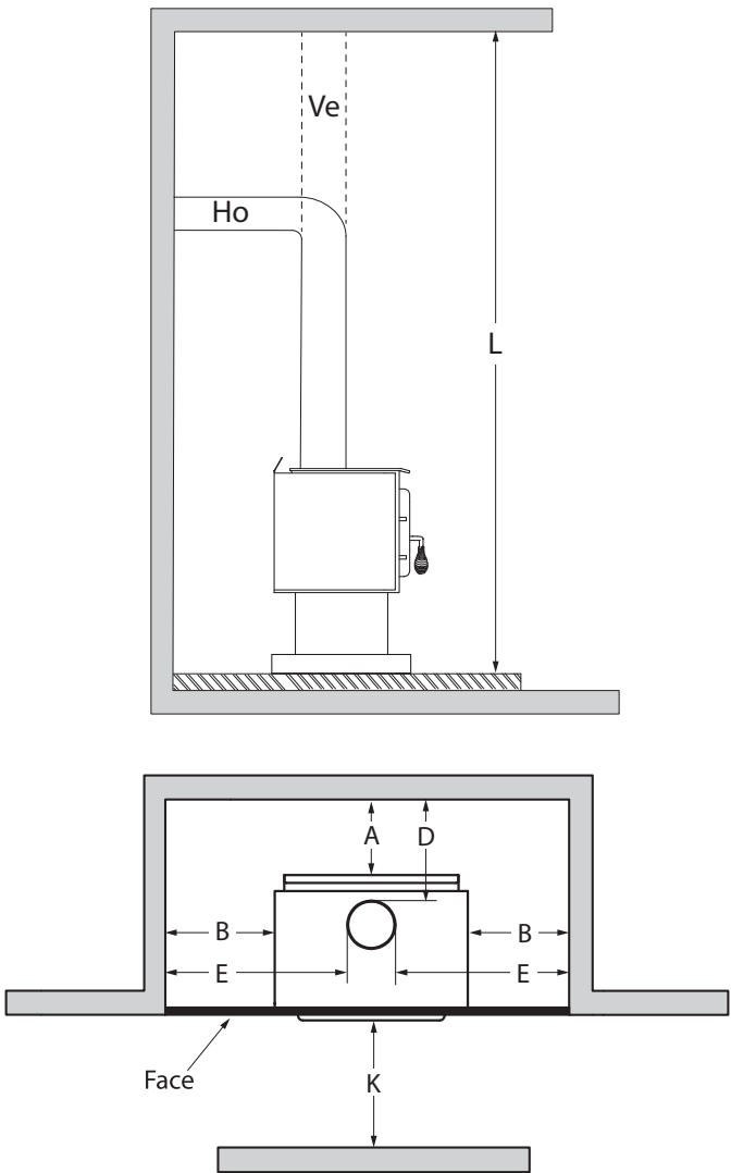
Figure 13: Clearances -Alcove
