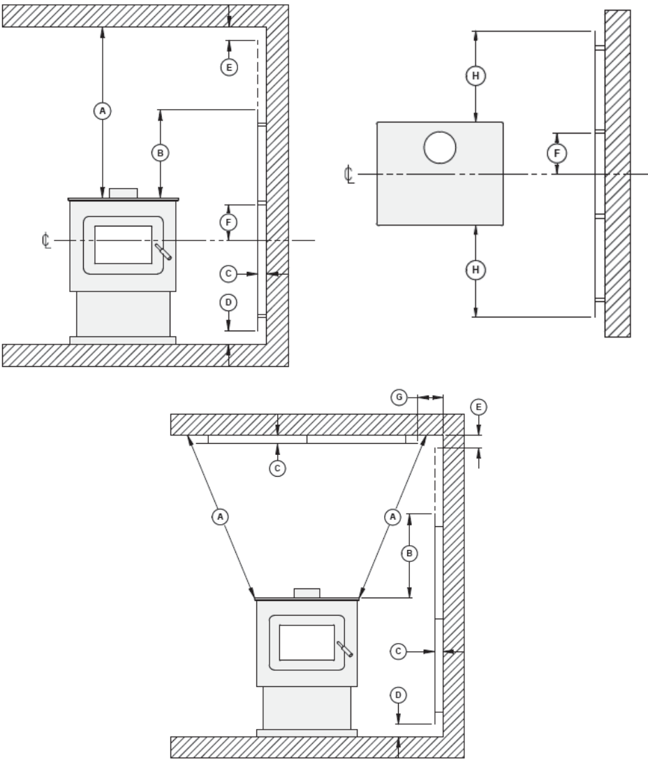
Clearances for shield construction
